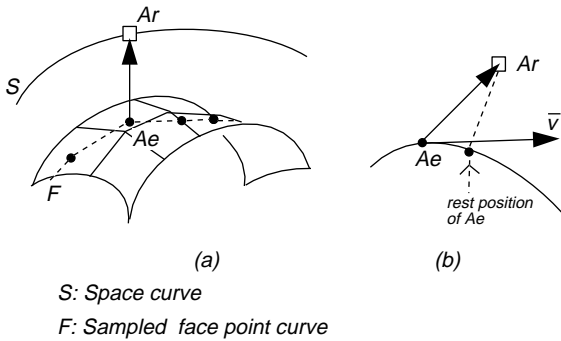
Figure 4. Sliding a face-point curve along a polygon mesh to smooth it. (a) shows an attractor Ar on the space curve and an attractee Ae on the polygon mesh. (b) shows a 1-D version of the curve and the rest position of Ae .
